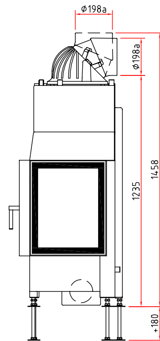
Anschlüsse
