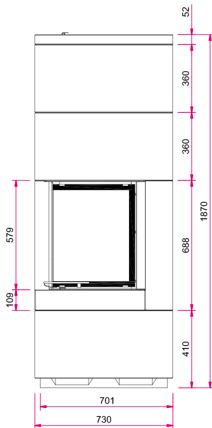
Front view, scale 1:20
