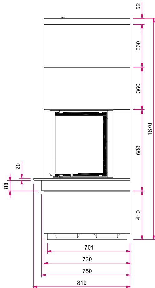
Front view, scale 1:20
