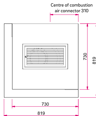
Top view, scale 1:25
