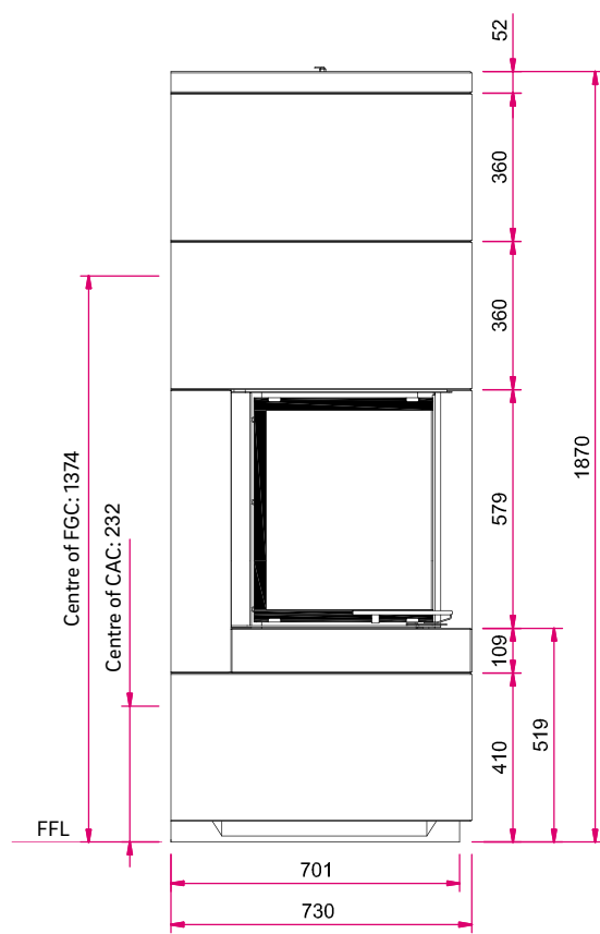
Left side view scale 1:20
