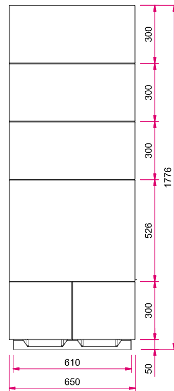
Left side view scale 1:20
