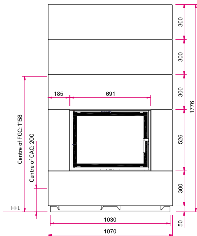
Front view, scale 1:20
