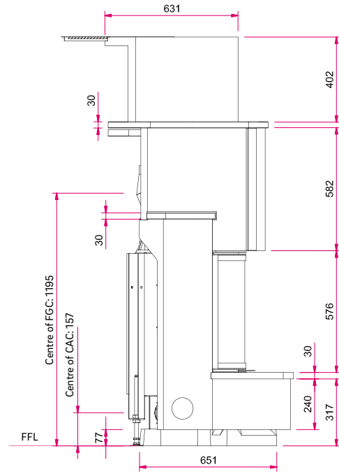
Left side view scale 1:25
