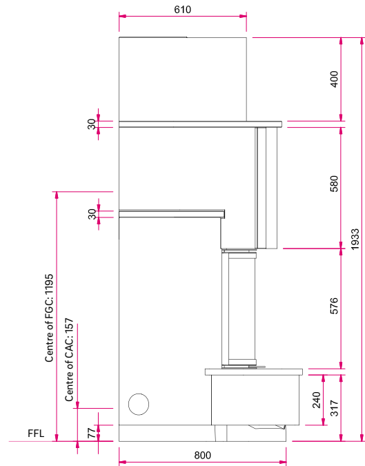
Left side view scale 1:25
