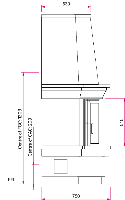
Left side view scale 1:20
