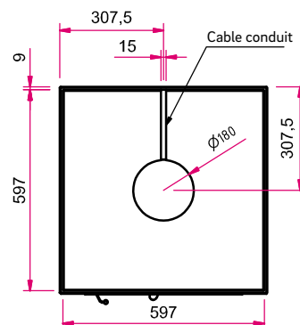
Screed recess (view of underside) scale 1:20
