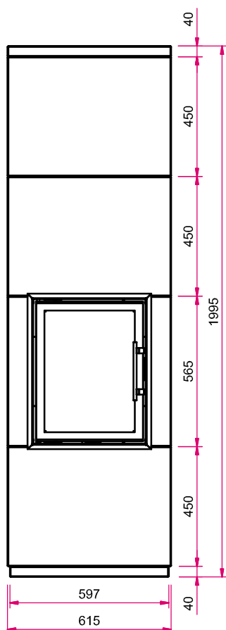
Front view, scale 1:20
