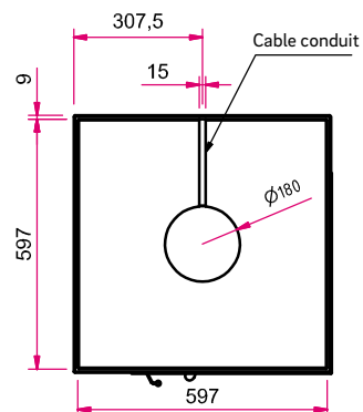
Screed recess (view of underside) scale 1:20
