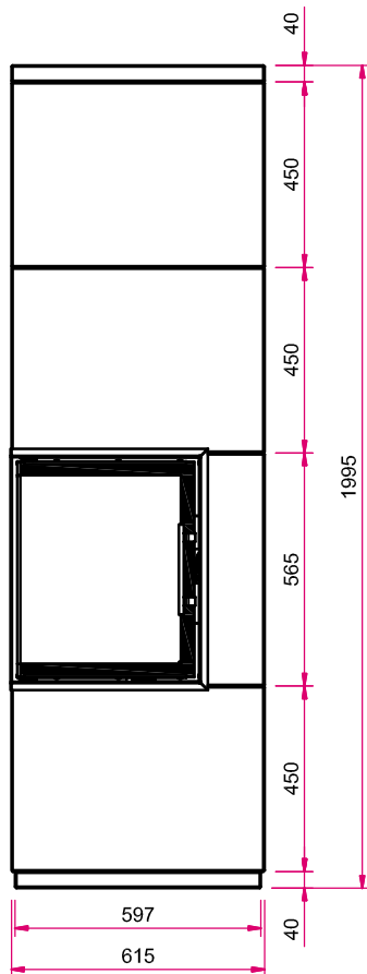
Front view, scale 1:20
