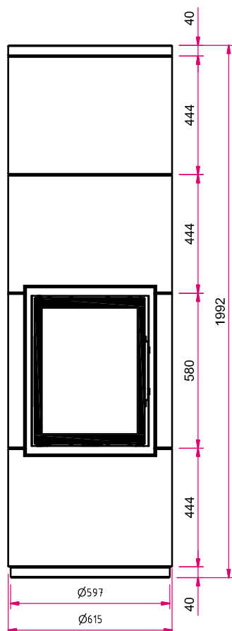
Front view, scale 1:20
