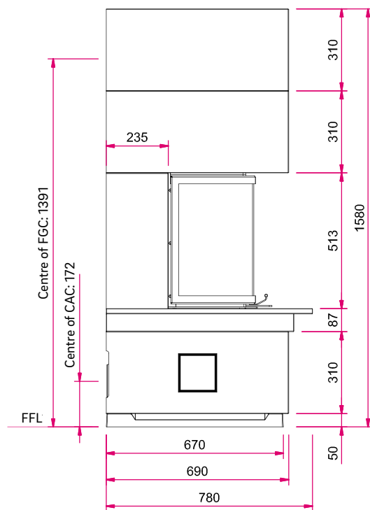
Left side view scale 1:20
