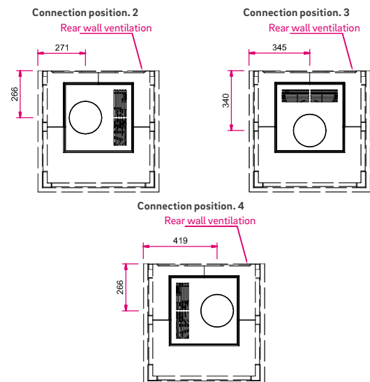
Top view, scale 1:30
