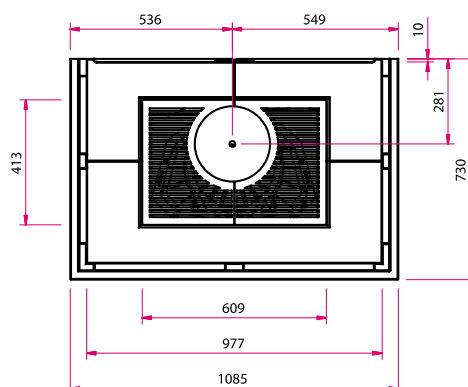
Top view, scale 1:25
