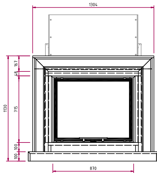
Front view, scale 1:25
