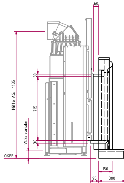
Left side view, scale 1:25
