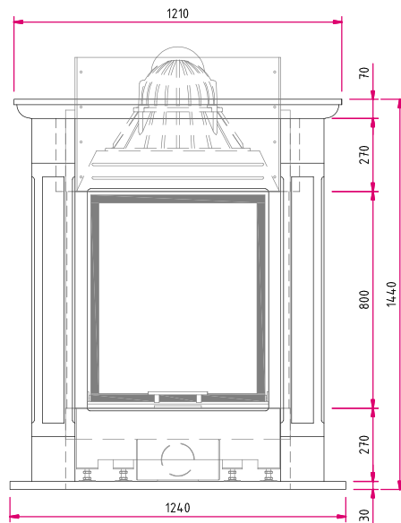
Front view, scale 1:25
