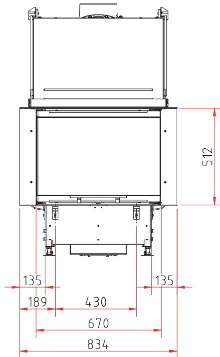
Front view, scale 1:20
