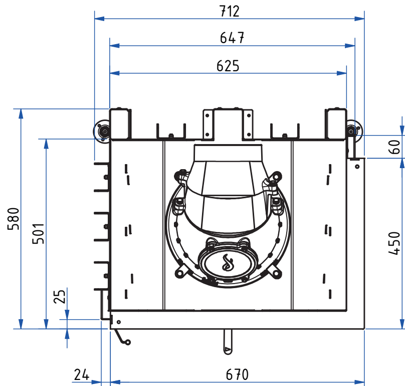
Top view, scale 1:10
