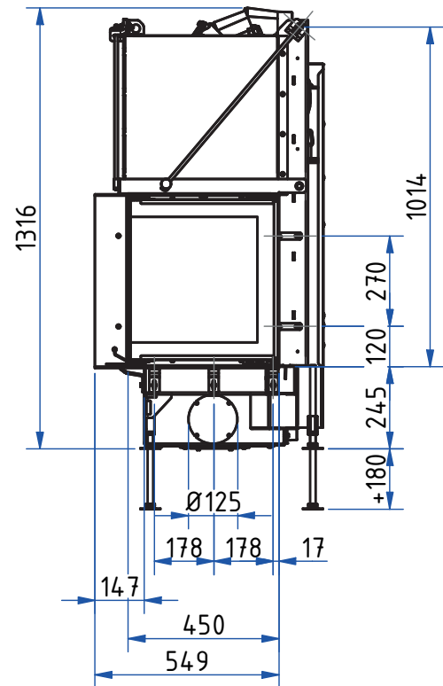
Side view, scale 1:20
