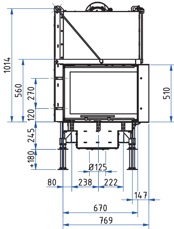
Front view, scale 1:20
