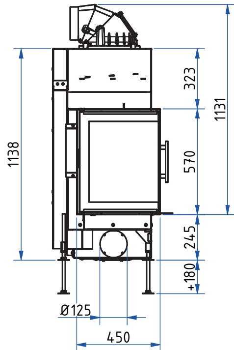
Side view, scale 1:20
