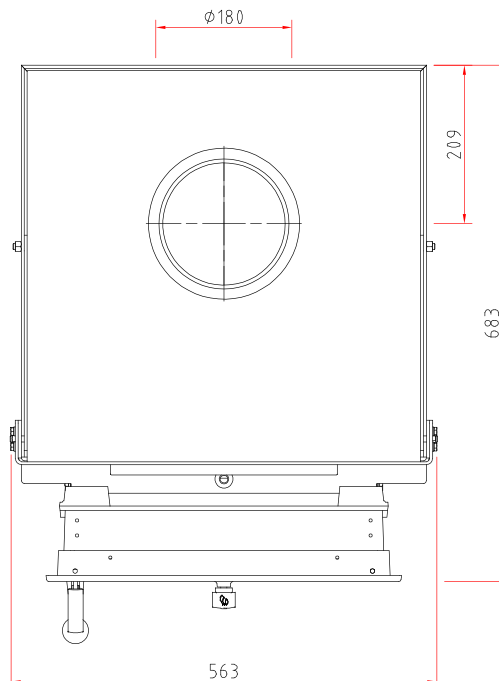
Top view, scale 1:10
