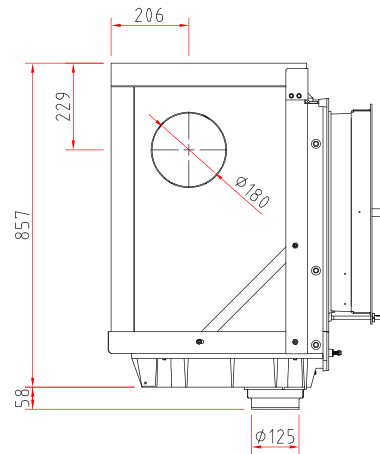
Side view, scale 1:20
