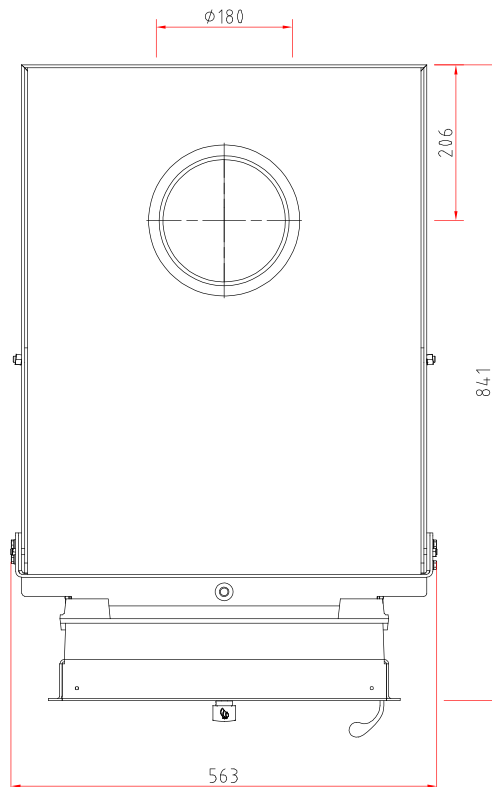
Top view, scale 1:10
