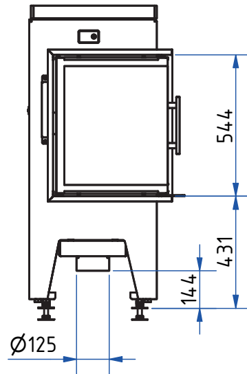
Side view with rotary chimney for wall and ceiling connection, scale 1:20
