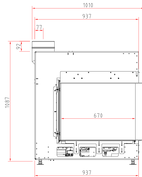
Side view, scale M 1:20
